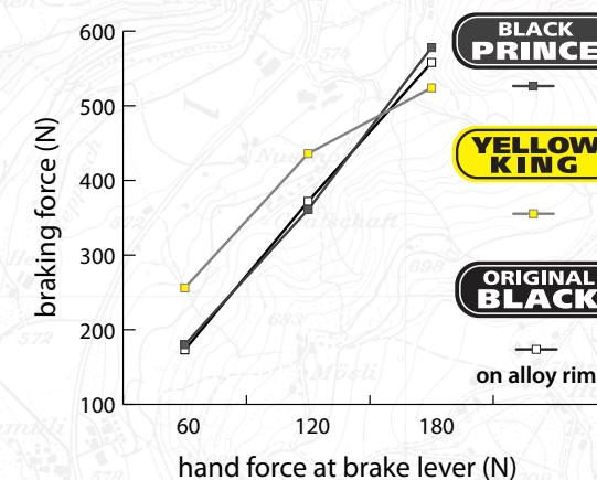
lever force vs. braking force
