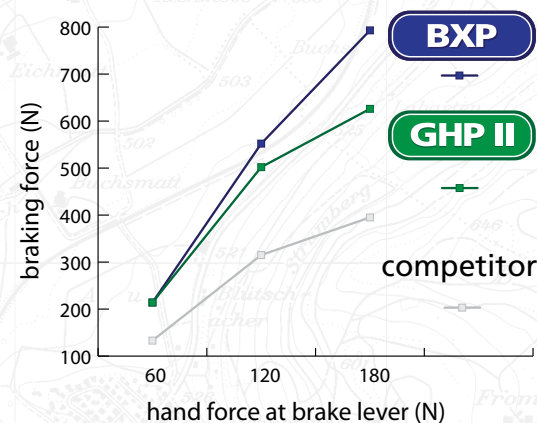
lever force vs. braking force
