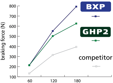
HAND FORCE at brake lever (N)
